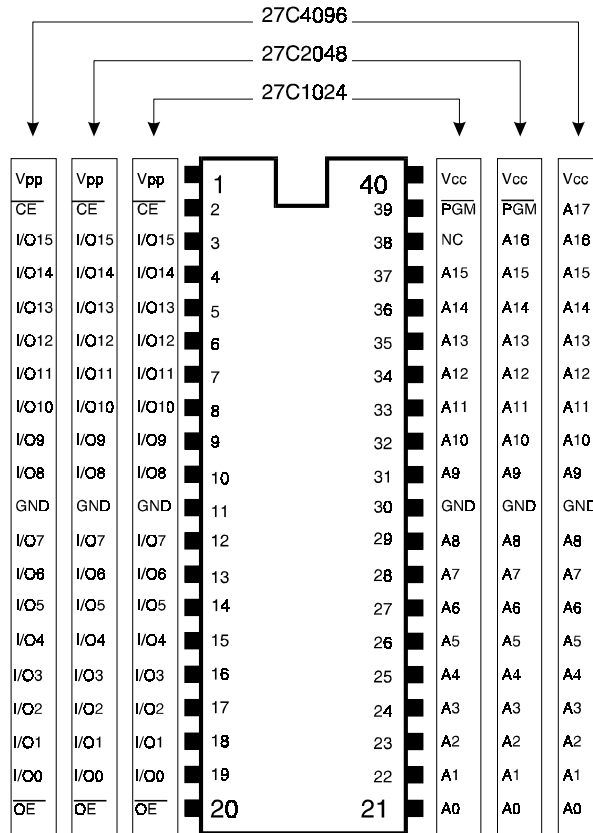
JEDEC Standard EPROM Pinouts (27C1024 - 27C4096)
