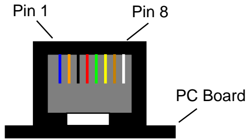
RJ-45 Socket - mounted on unit
