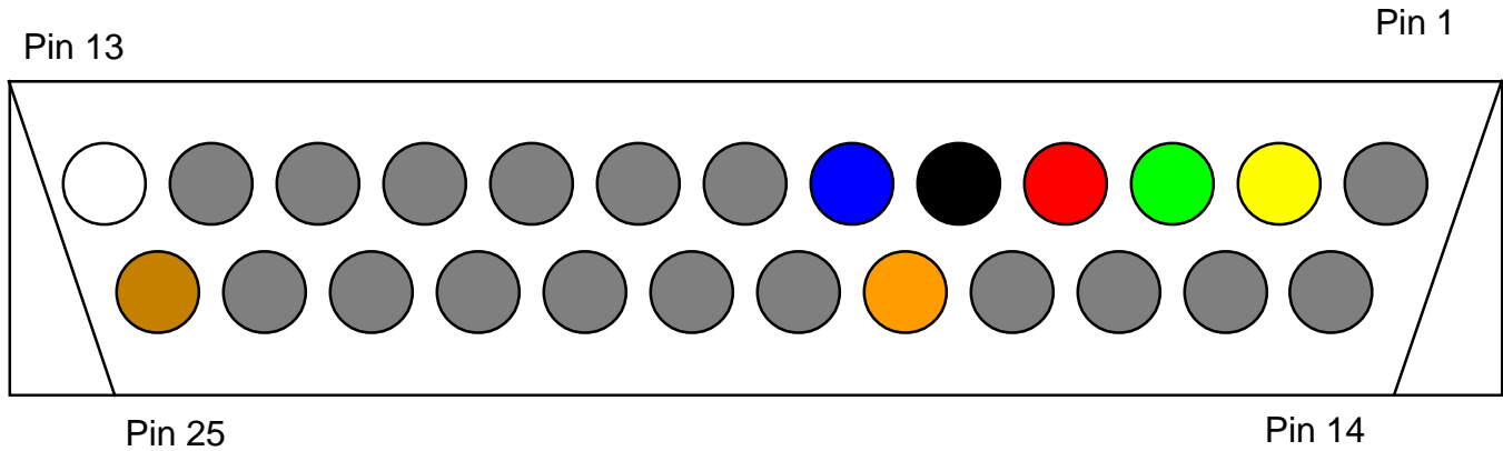
DB25 Connector - back view
